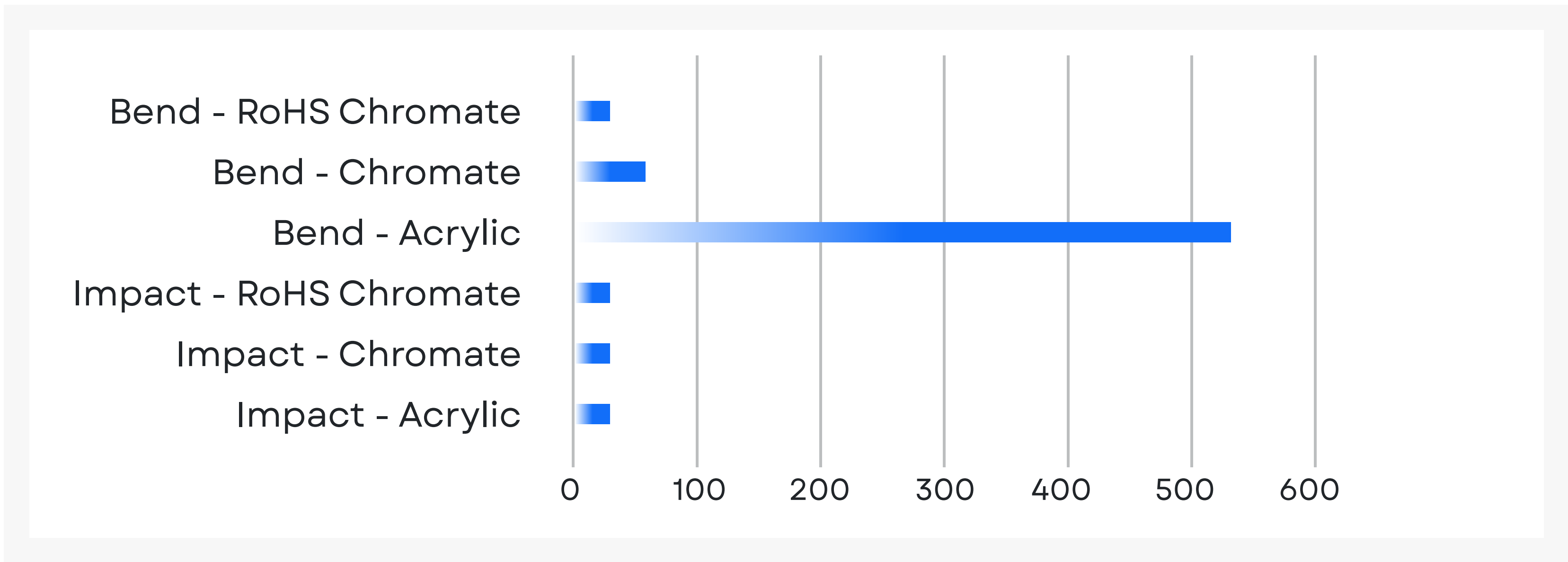
Figure 4. ASTM B117-18 Salt Spray test results on formed samples
