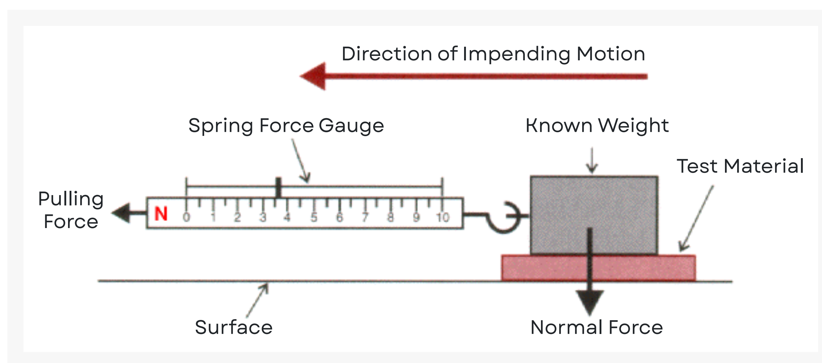
Figure 2. ASTM D1894-mod Friction Test sample and test sled
