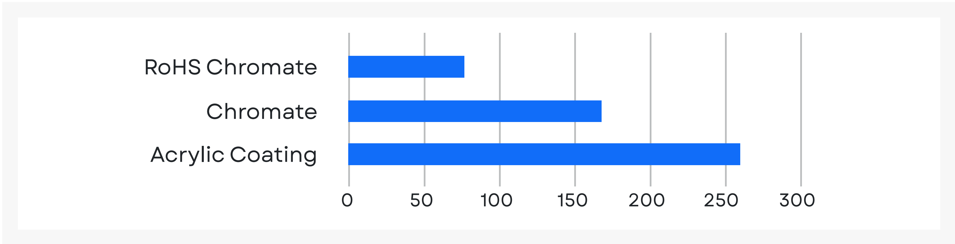
Figure 1. ASTM B117-18 Salt Spray test results on flat samples
