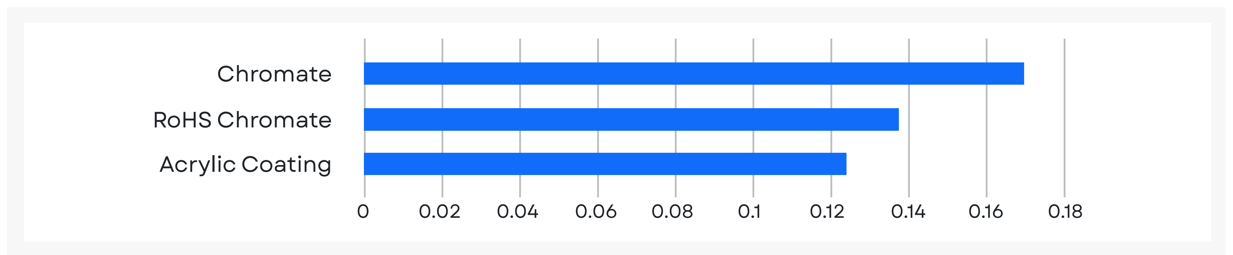
Figure 3. ASTM D1894-mod Coefficient of Friction test results on flat samples
